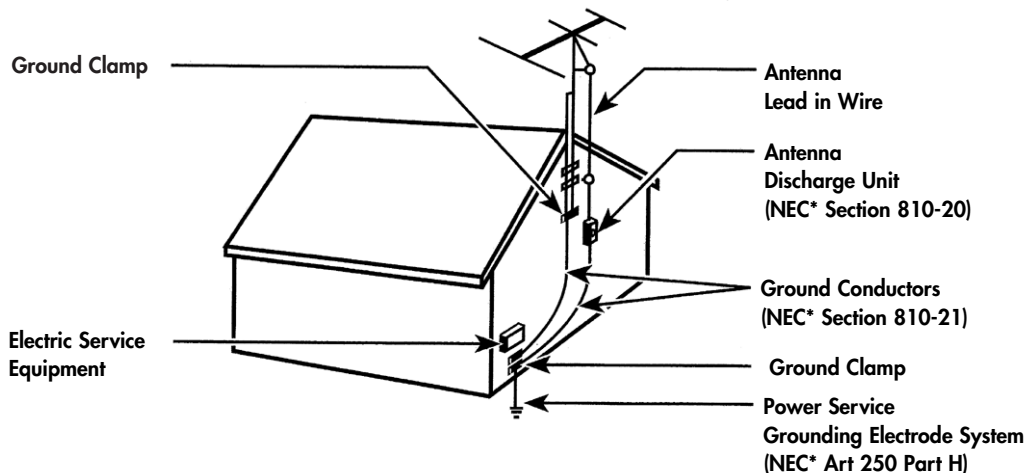
Antenna Grounding According to the National Electrical Code
